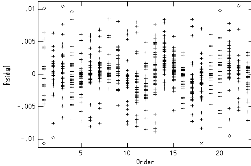
Figure 15: The final fit.
