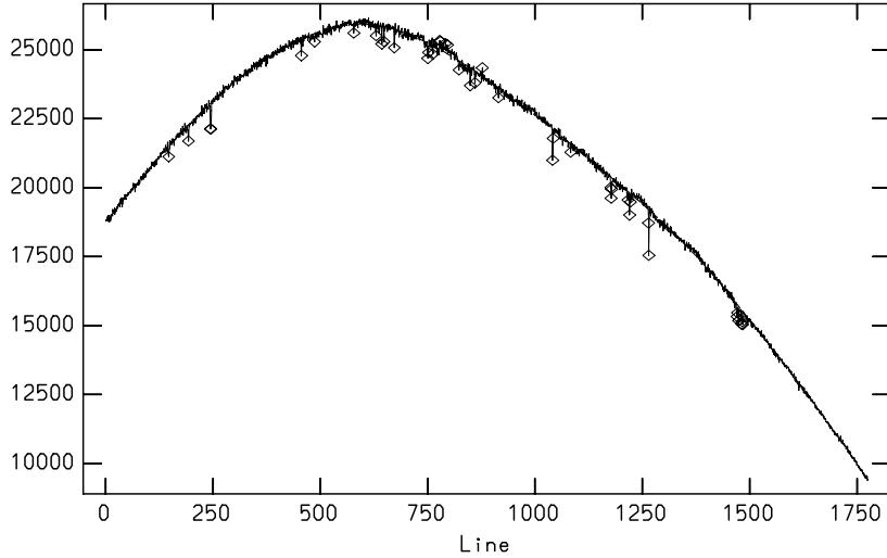
Figure 5: Fit along the dispersion of the general spectral shape.
