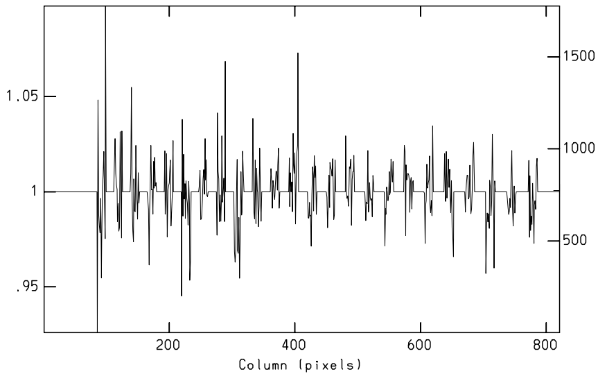
Figure 6: A plot of the output image from apflatten perpendicular to the dispersion. The regions between the orders have been set to 1; the data inside the apertures have been normalized to 1 with the large scale gradients removed.
